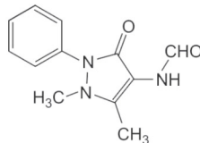
A. 4-(formyloamino)-1,5-dimetylo-2-fenyl-2,3-dihydro-1H-pirazol-3-on,
